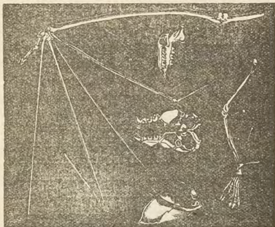
VESPERTILIO PARISIENSIS. A Bat of the Eocene.
